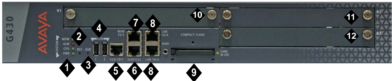
Figure 1: The Avaya G430 Media Gateway Chassis
