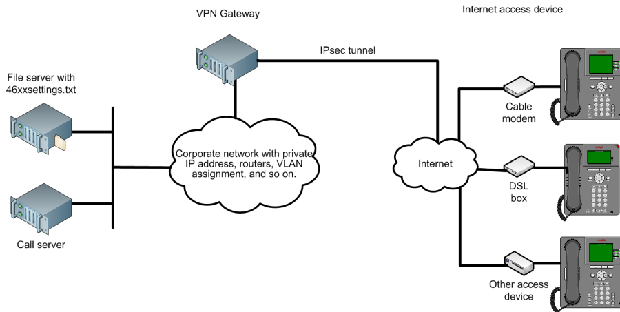
Figure 1: VPN configuration
